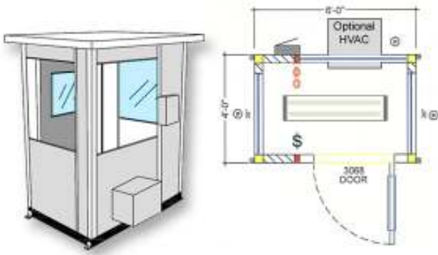
4' x 6' x 8' High—Exterior Guardhouse
