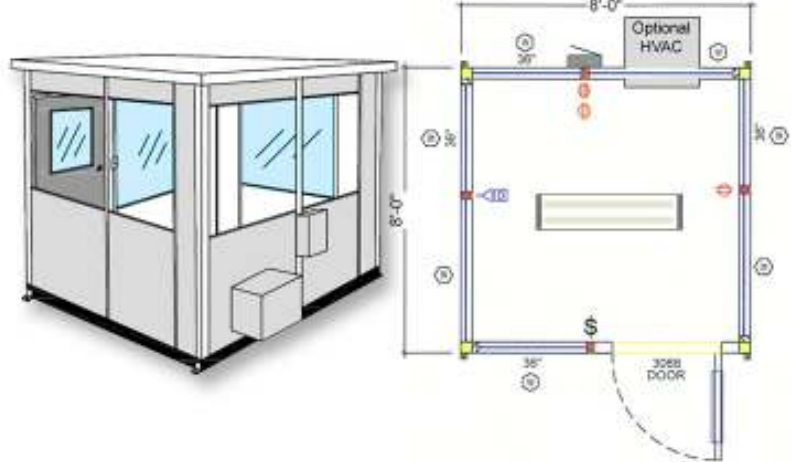
8' x 8' x 8' High—Exterior Guardhouse
