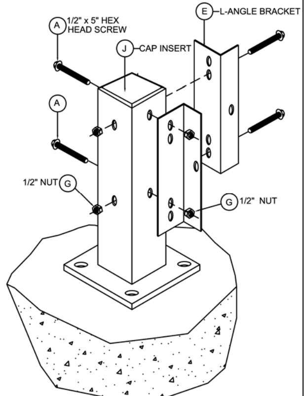
CORNER POST
