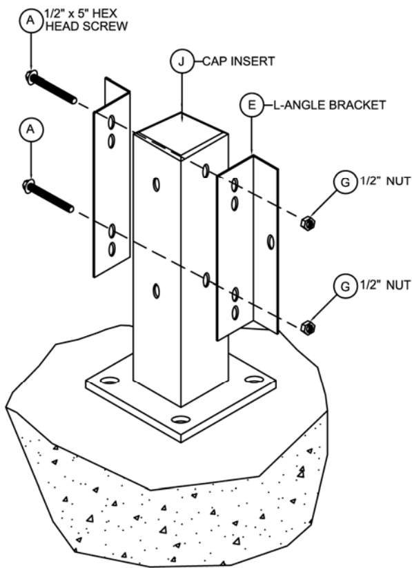
INTERMEDIATE POST
