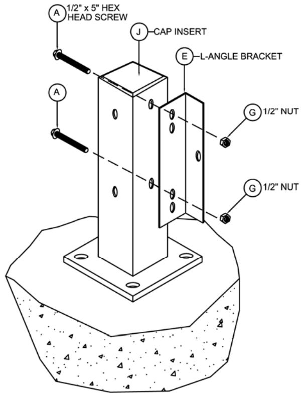
END POST
